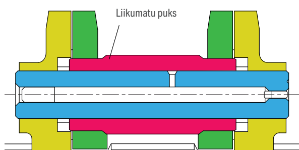
Standardne roomik
