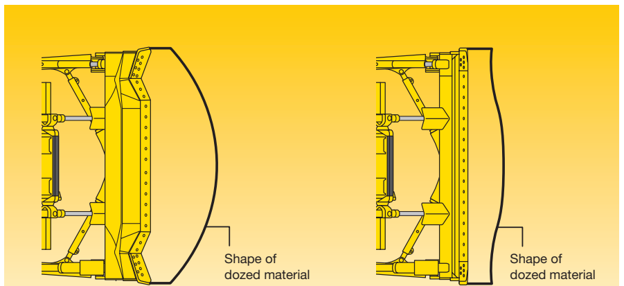
Up to 15% higher productivity with the improved Sigadozer® blade (left), compared to conventional Semi-U blade (right)
