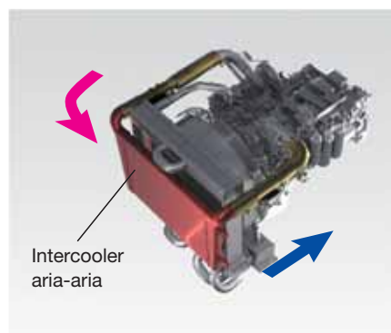
Intercooler aria-aria
